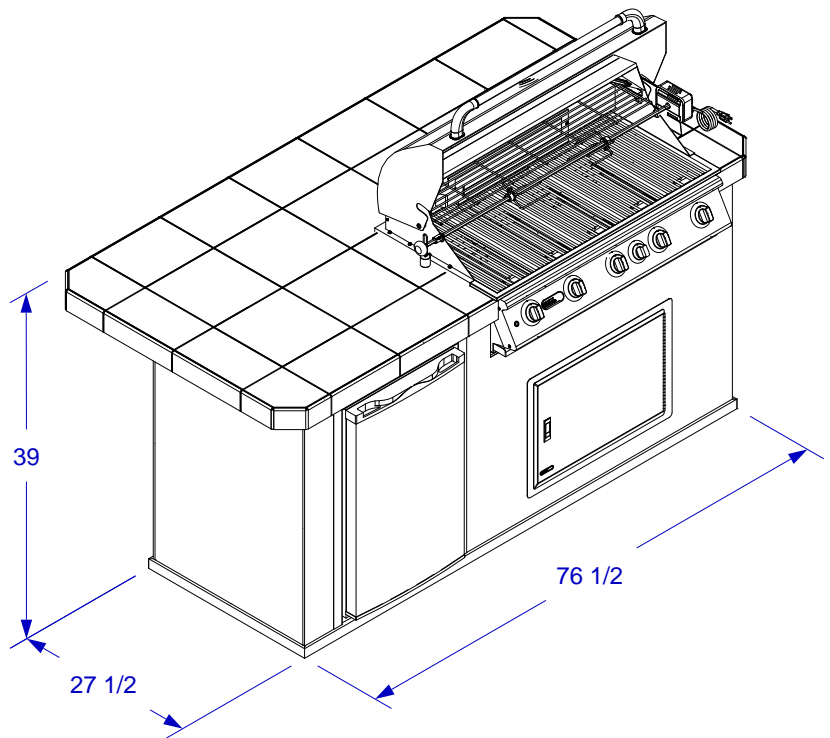
ISOMETRIC VIEW
