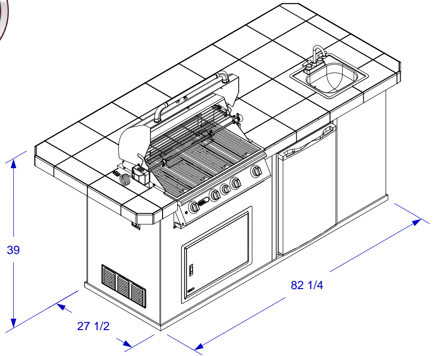
ISOMETRIC VIEW
